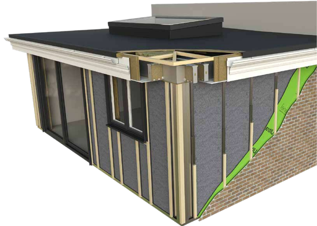
hup! Flat Roof with Flat Skylight.
